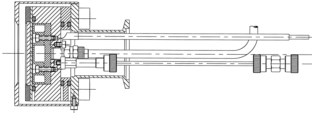
SIDE VIEW OF UTILITY CONNECTIONS
