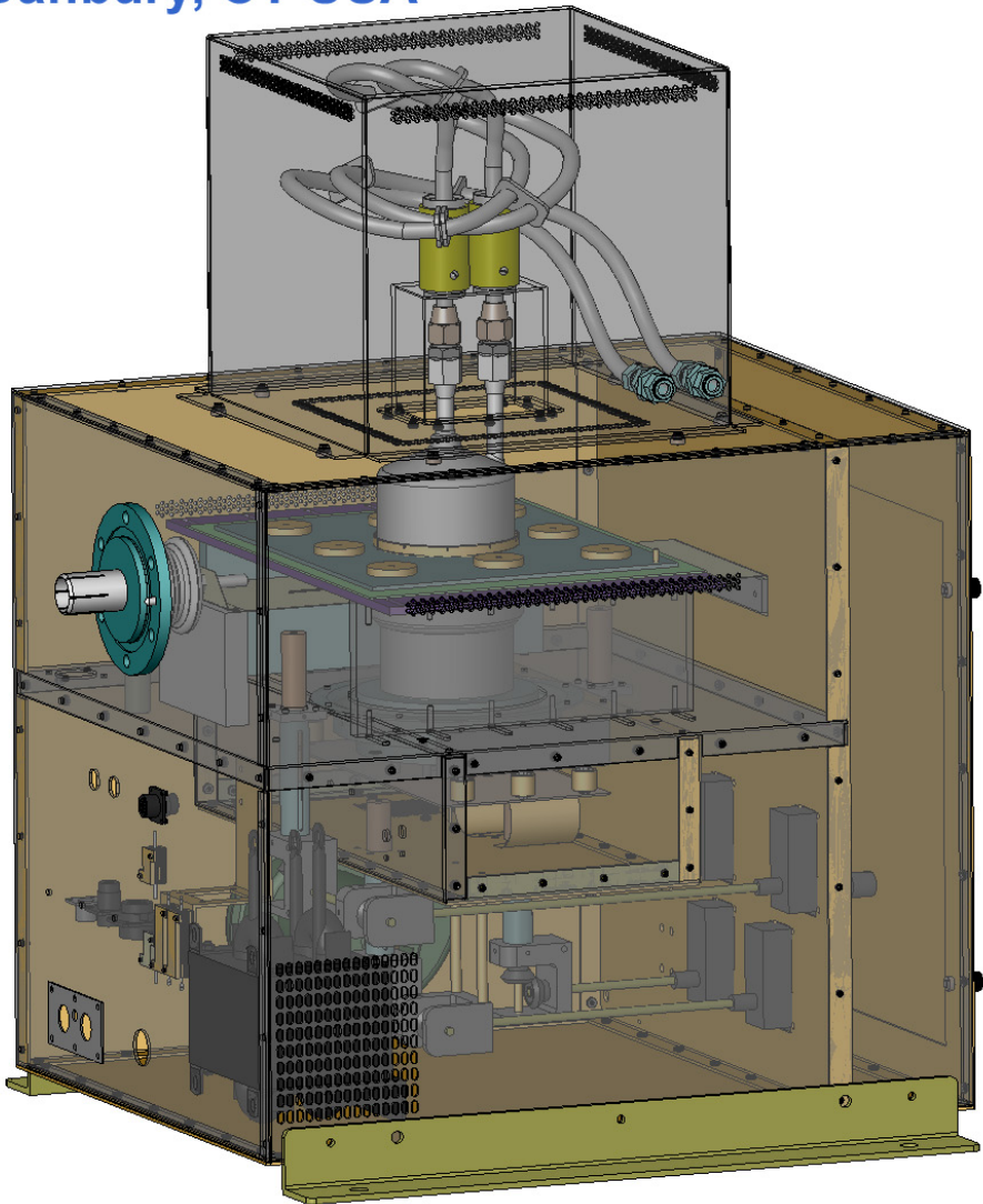
Model HVT20K150 RF Power Generator Head
