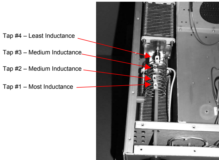
PB3 Matching Network Section Inductor Tap Selection
