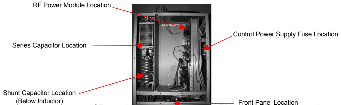
PB3 Chassis top view
